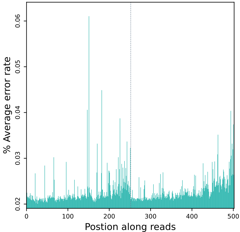
Error rate distribution along reads (R10818)
